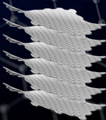
Self-assembly by designed intermolecular interactions
